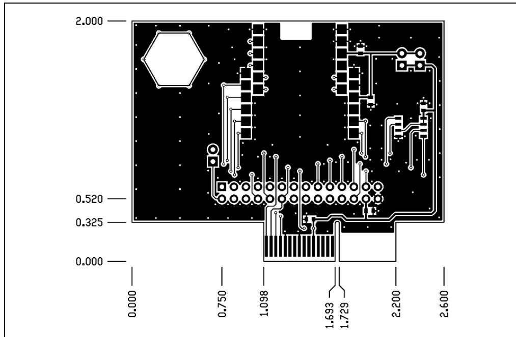
FIGURE A-3: MRF24J40ME PICtail™/PICtail PLUS DAUGHTER BOARD TOP COPPER
