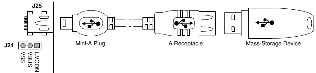
Figure 2-20. USB Mass Storage Device Connection
