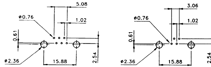
PC Board Layout PC Board Layout
