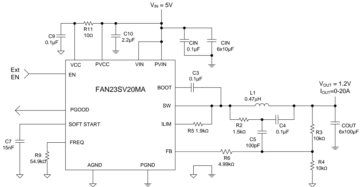
Figure 2. Typical Application with V_{IN}=5\text{ V}
