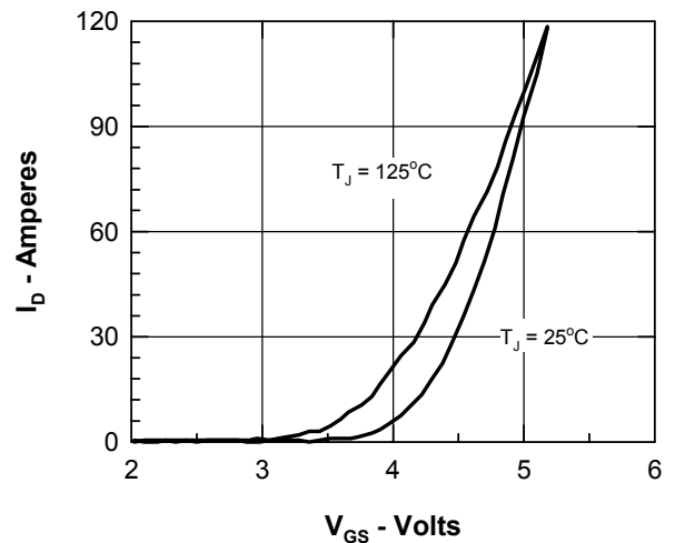
Figure 6. Admittance Curves
