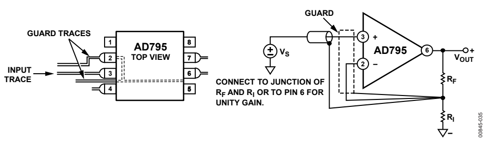
Figure 35. Guard Scheme—Follower
