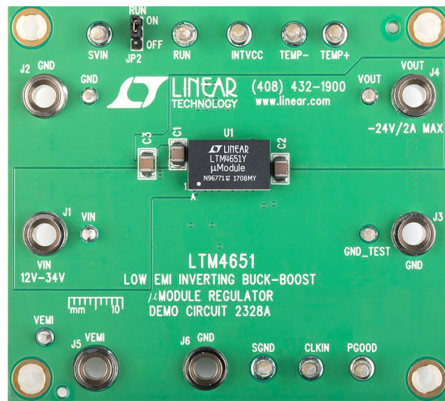
DC2328A Top View
