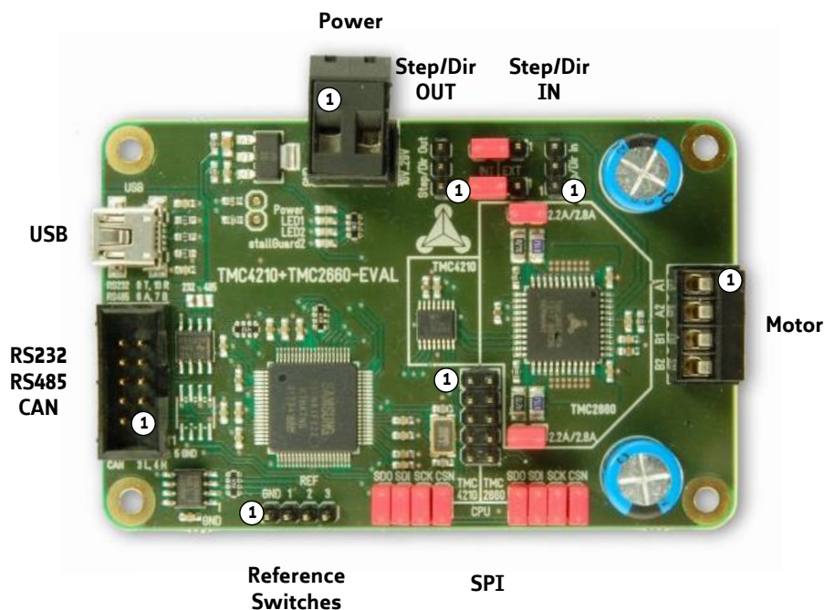
Figure 3.2 Connectors of TMC4210+TMC2660-EVAL
