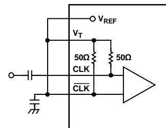
CONNECT V_T , V_{REF} , AND \overline{\text{CLK}} . PLACE A BYPASS CAPACITOR FROM V_T TO GROUND. ALTERNATIVELY, V_T , V_{REF} , AND CLK CAN BE CONNECTED, GIVING A CLEANER LAYOUT AND A 180^\circ PHASE SHIFT. Figure 22. Interfacing to AC-Coupled Single-Ended Inputs
