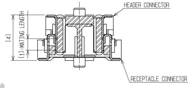
CROSS CUT SECTION - GROUND (5:1)
