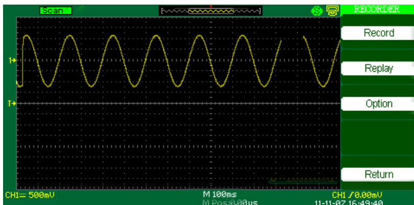
Figure 79 - Record Screen
