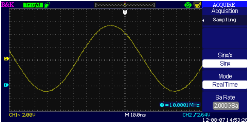
Figure 39 - Acquire Menu
