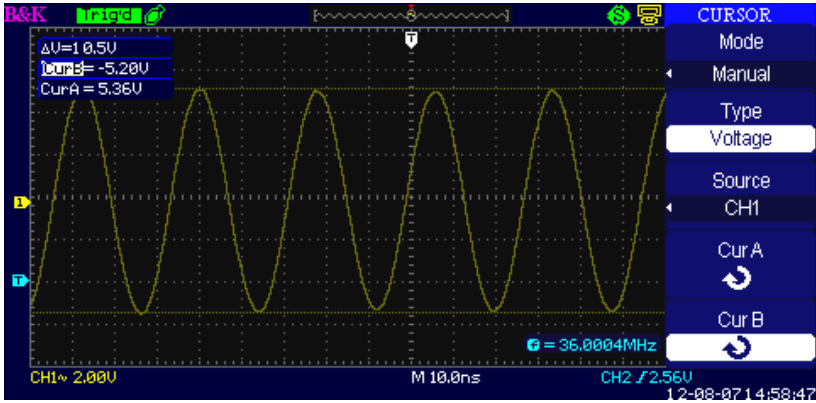
Figure 48 - Cursor Menu
