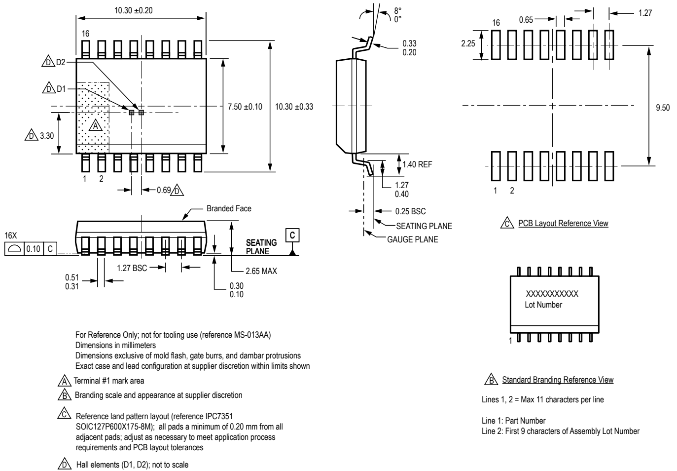
Figure 15: Package LA, 16-pin SOICW
