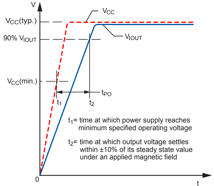
Figure 11: Power-On Time ( t_{PO} )
