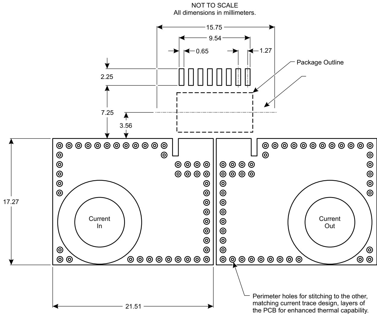
Figure 14: High Isolation PCB Layout
