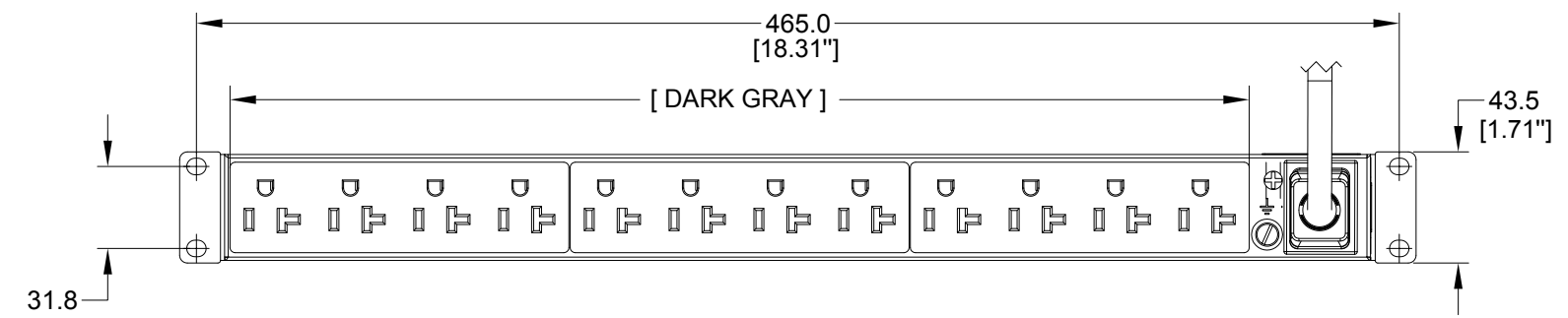
FRONT VIEW
