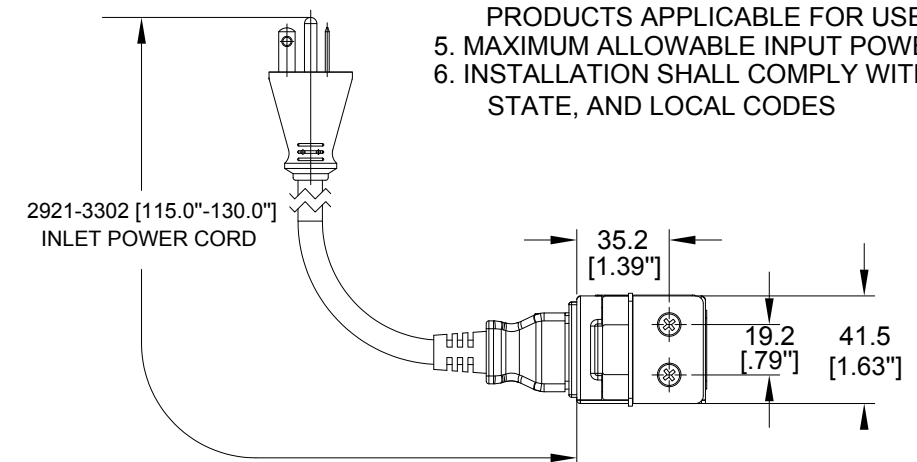
SIDE VIEW
