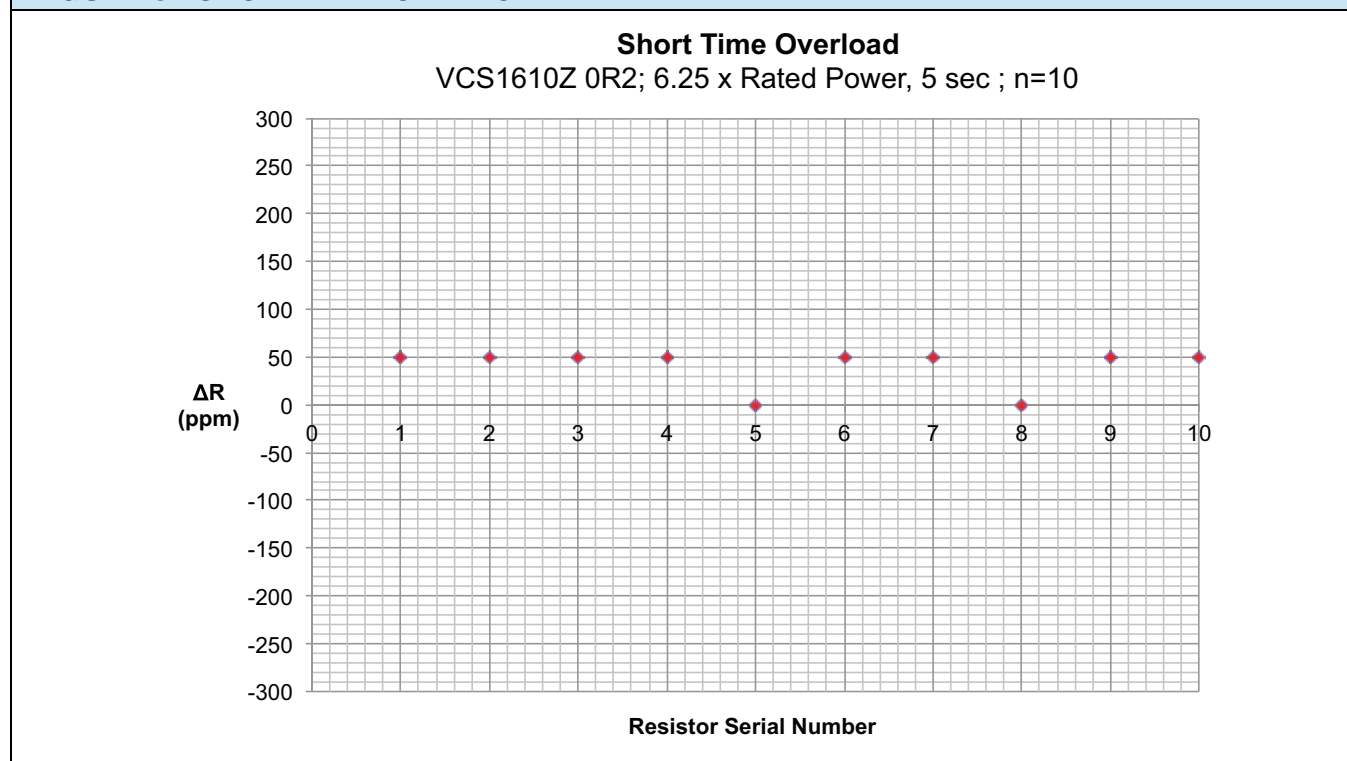
FIGURE 8 - SHORT TIME OVERLOAD
