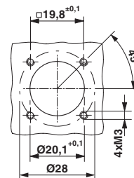
Installation dimensions RF-...N8AWA00, RF-...N8AWB00
