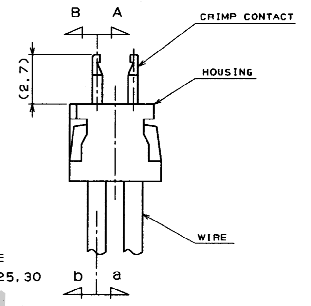
CRIMP CONTACT INSERTION DRAWING
