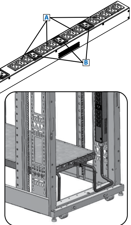
An 8-position plug installs directly to the ATS mating receptacle on the back of the unit.
