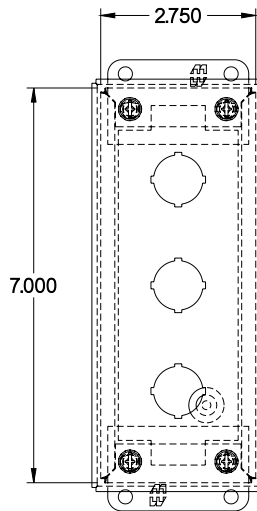
FRONT VIEW
