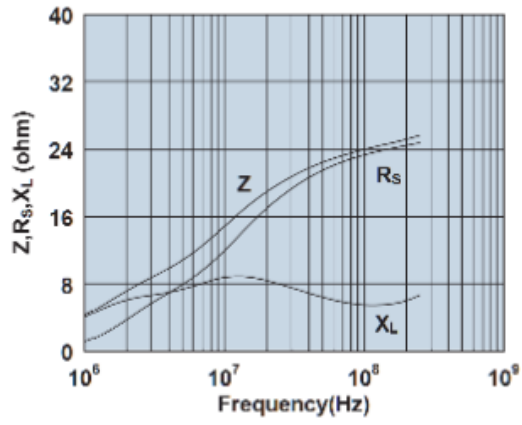
Impedance, reactance, and resistance vs. frequency.
