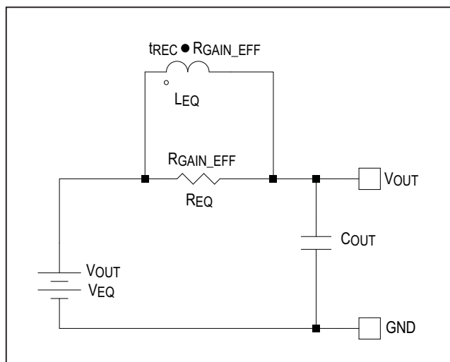
Figure 4. Averaged Small-Signal Equivalent Circuit of Regulator
