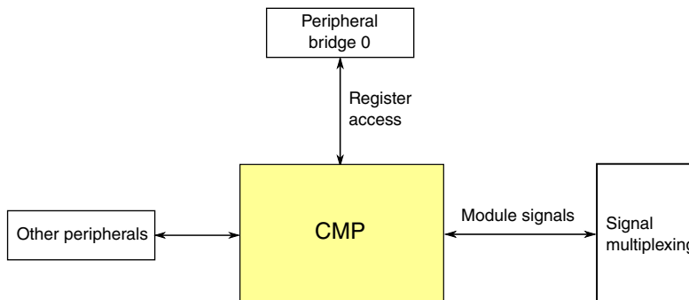
Figure 3-31. CMP configuration
