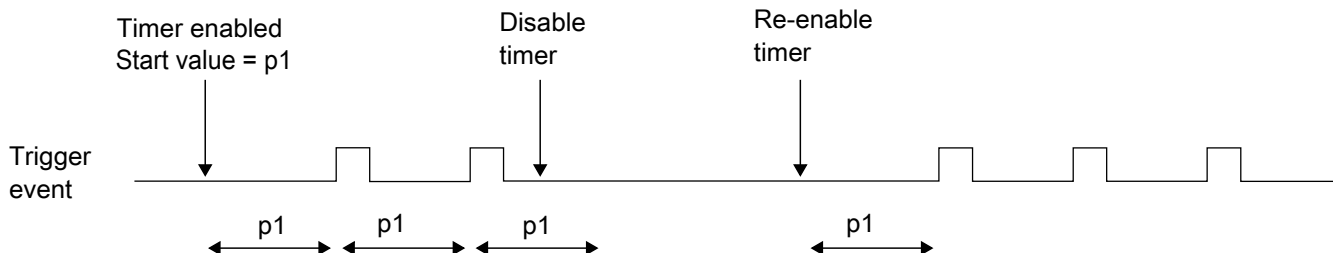
Figure 39-2. Stopping and starting a timer
