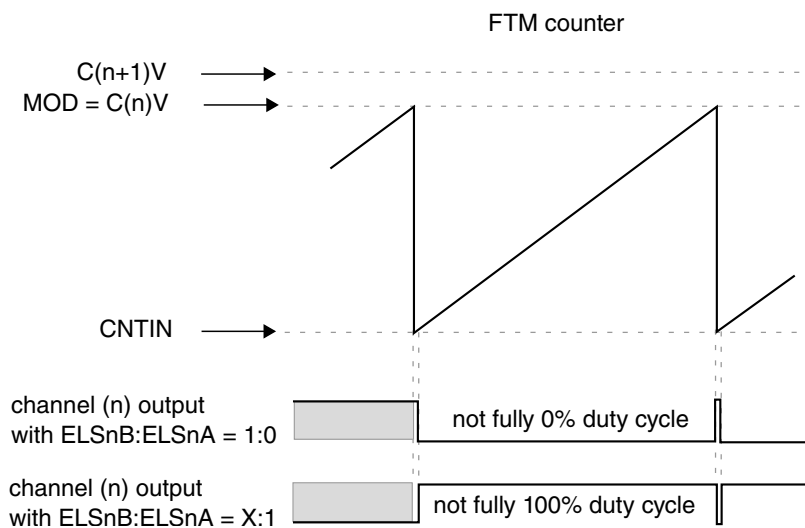
Figure 38-40. Channel (n) output if (C(n+1)V > MOD and (CNTIN < C(n)V = MOD)
