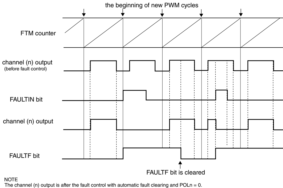
Figure 38-73. Fault control with automatic fault clearing
