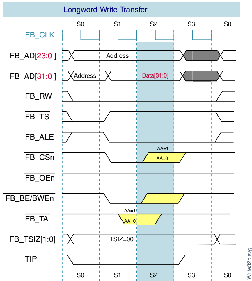
Figure 30-12. Longword-Write Transfer
