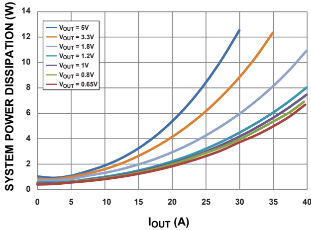
SYSTEM POWER DISSIPATION
