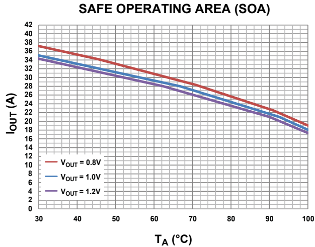
Conditions: V_{DDH} = 5V
