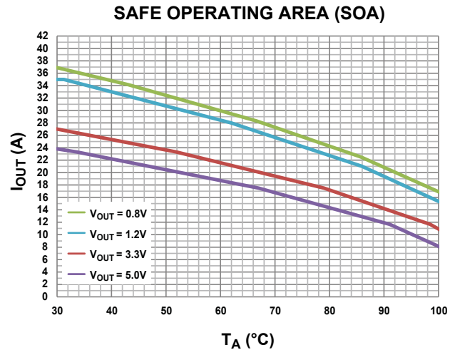
Curve indicates T_J = 125^\circ C or I_{OUT} = I_{MAX} , whichever happens first.
