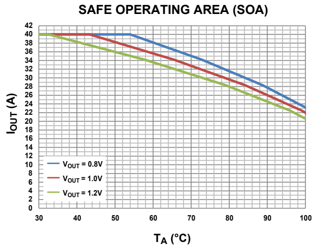
Conditions: V_{DDH} = 5V 200 LFM
