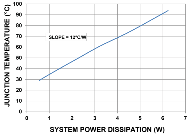
JUNCTION TEMPERATURE vs. SYSTEM POWER DISSIPATION
