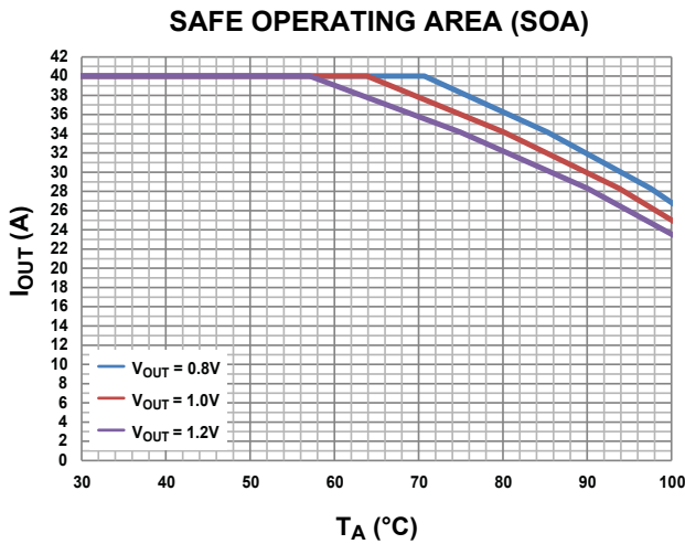
Conditions: V_{DDH} = 5V 400 LFM
