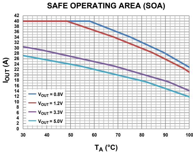
Conditions: 200 LFM Curve indicates T_J = 125^\circ C or I_{OUT} = I_{MAX} , whichever happens first.
