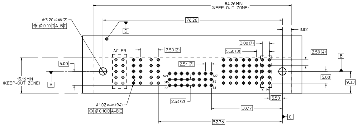
RECOMMENDED PC BOARD LAYOUT & KEEP-OUT ZONE
