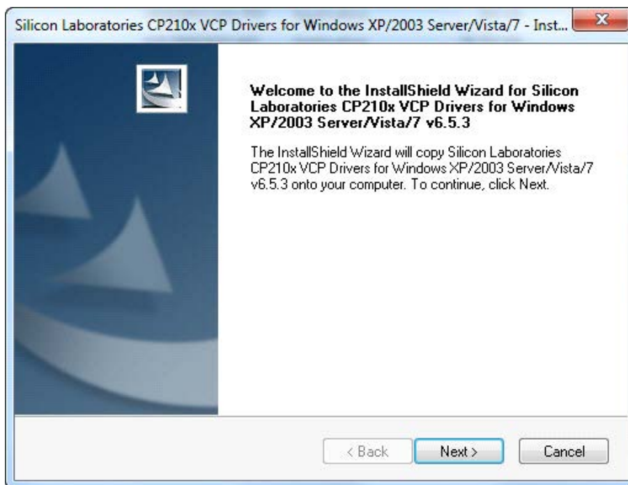
Figure 5. InstallShield Wizard
