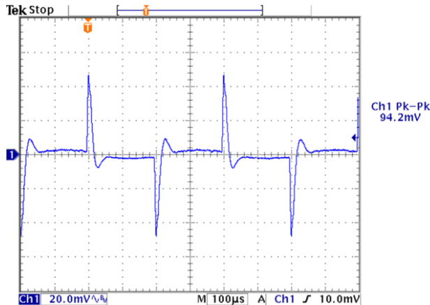
Figure 10 Transient Response with Regulation set to 0 mV/A.
