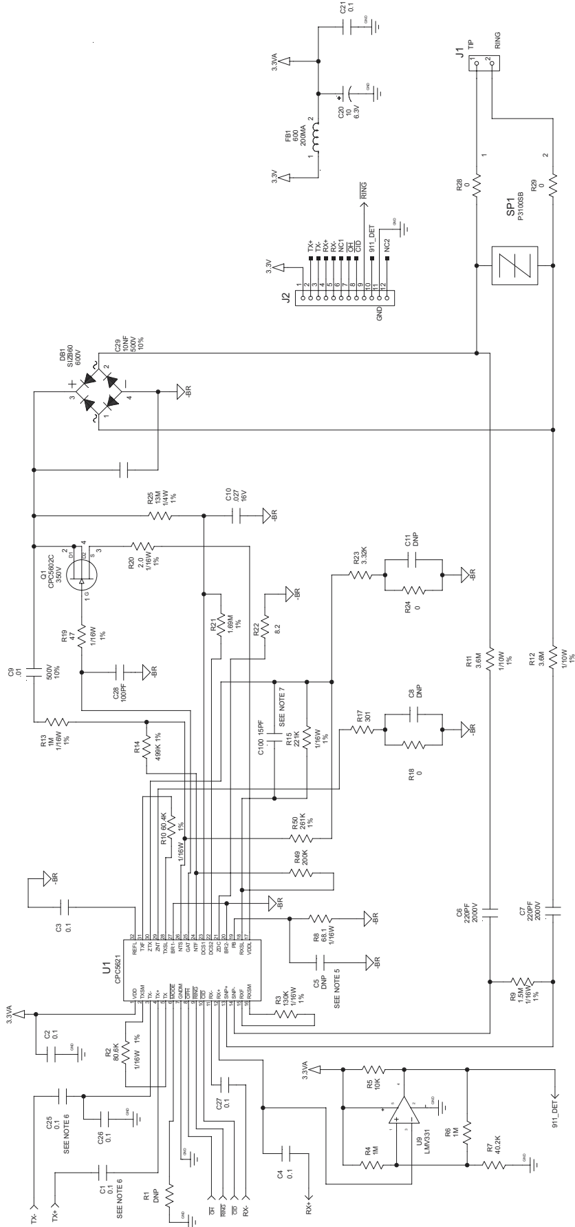
Figure 8. CPC5621-EVAL-RDL Schematic
