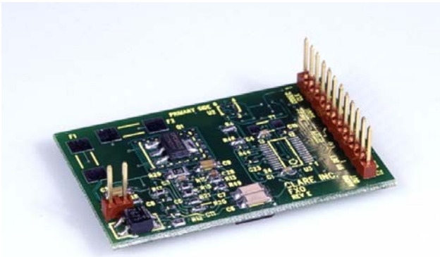
Figure 1. LITELINK III Evaluation Board, Primary (Top) View
