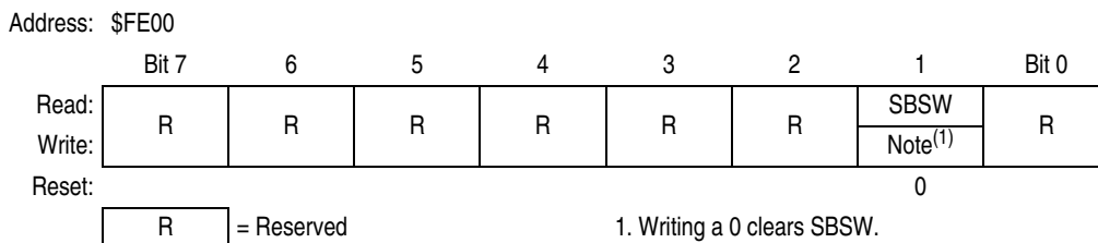
Figure 15-7. Break Status Register (BSR)
