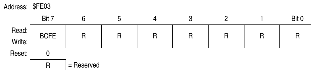
Figure 15-8. Break Flag Control Register (BF CR)
