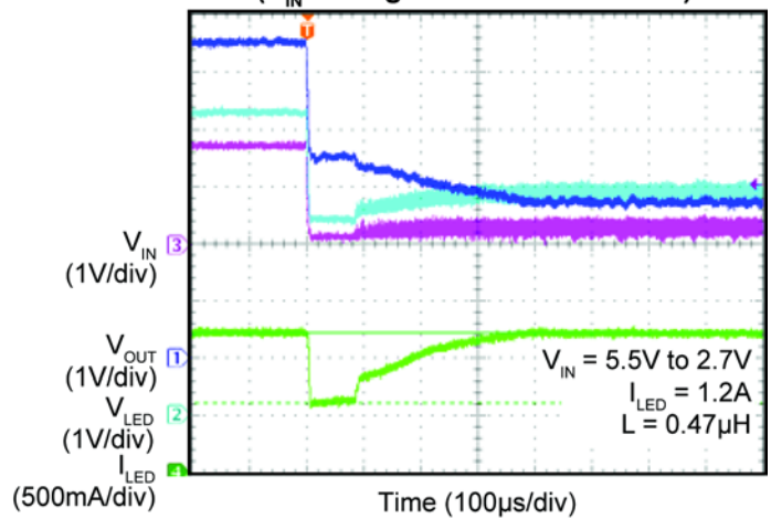
Line Transient ( V_{IN} Changes from 5.5V to 2.7V)
