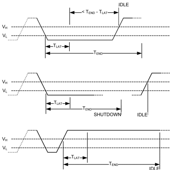
Figure 2. Abort, Shutdown and Idle Timing Waveforms
