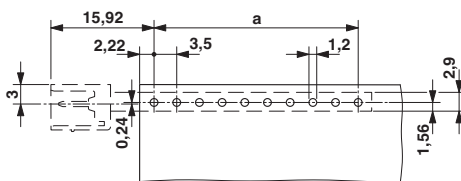
Drilling diagram
