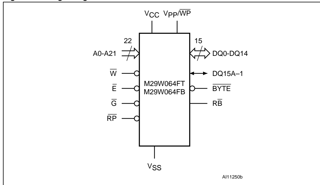
Figure 1. Logic diagram
