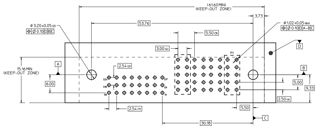
RECOMMENDED PC BOARD LAYOUT & KEEP-OUT ZONE
