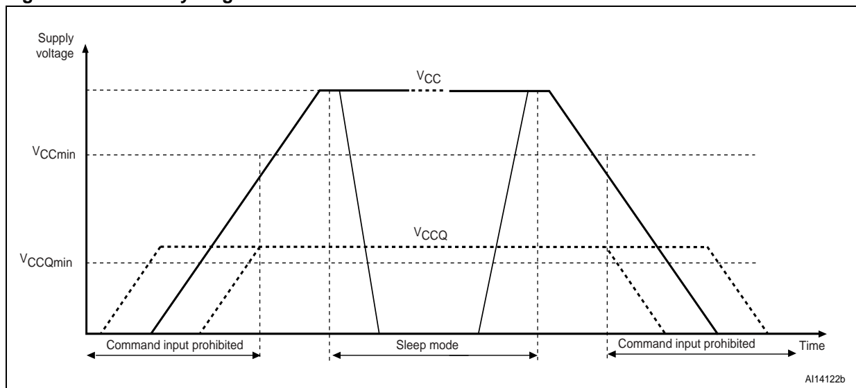
Figure 7. Power cycling
