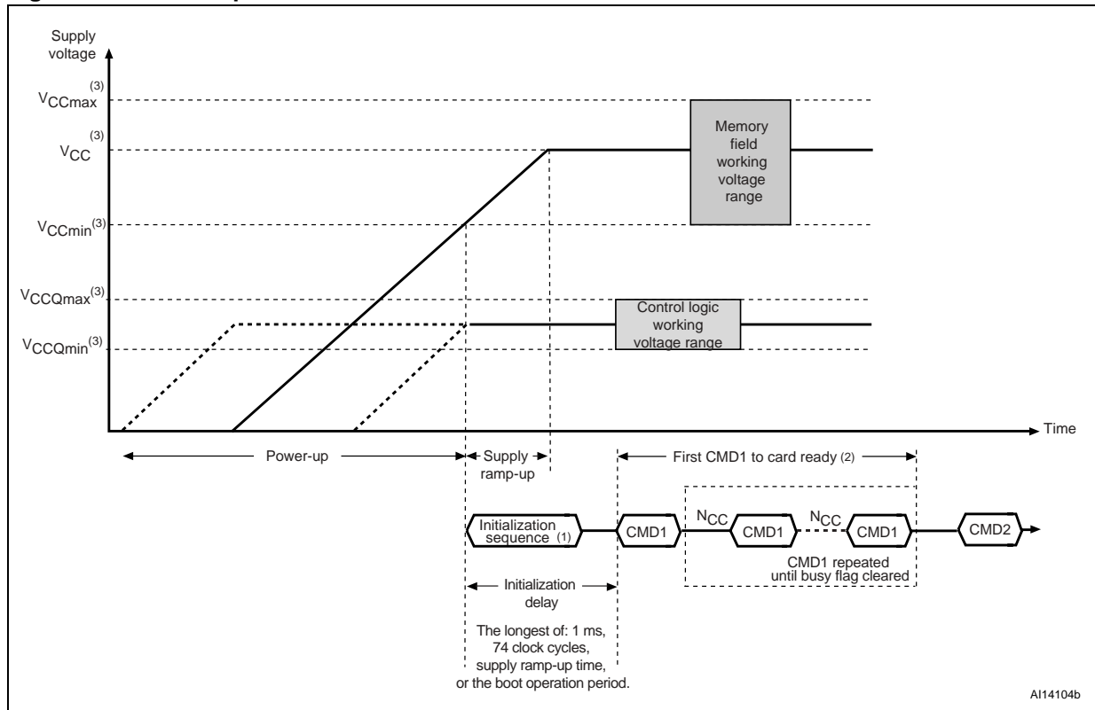
Figure 6. Power-up
