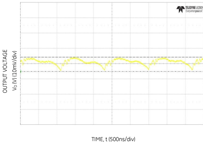
Figure 9. Typical output ripple ( C_o=2 \times 47 \mu\text{F} ceramic, V_{IN} = 12\text{V} , I_o = I_{o,max} ).
