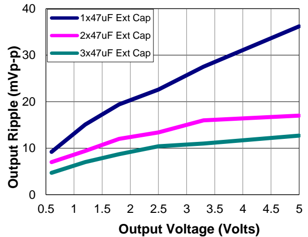
Figure 38. Output ripple voltage with external 1x47μF, 2x47 μF, or 3x47 μF ceramic capacitors at the output (3A load). Input voltage is 12V. Scope BW Limited to 20MHz.
