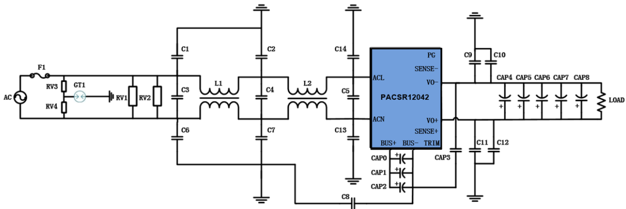
Figure 9: Application connection
