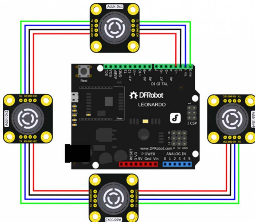
URM07 Cascade Connection
