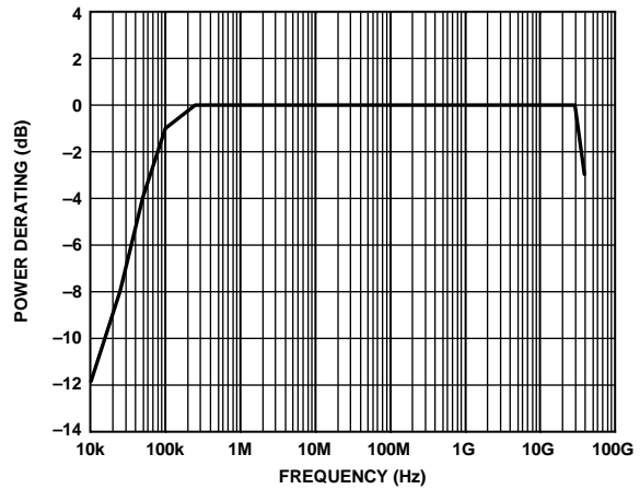
Figure 3. Power Derating for Terminated Path vs. Frequency, T_{CASE} = 85^{\circ}C
