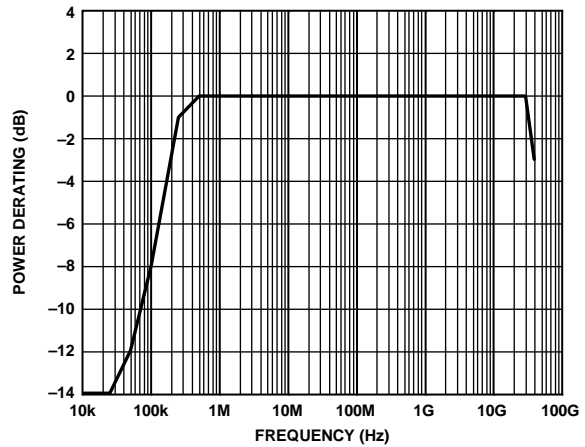
Figure 2. Power Derating for Through Path and Hot Switching vs. Frequency, T_{CASE} = 85^{\circ}C
