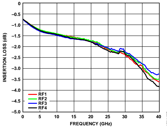
Figure 7. Insertion Loss vs. Frequency for RF1, RF2, RF3, and RF4
