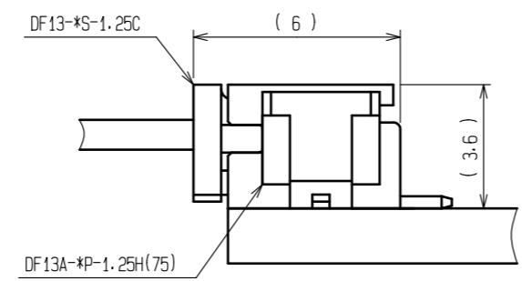
APPLICATION DRAWING
