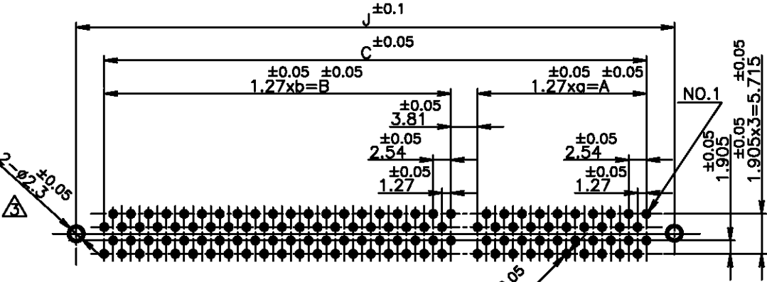
P.C. BOARD LAYOUT (CONNECTOR MOUNT SIDE)
