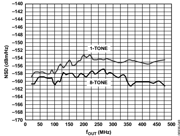
Figure 49. AD9780 One-Tone, Eight-Tone NSD vs. f_{OUT} in Baseband and Mix Modes, at 500 MSPS, FS = 20\text{ mA}
