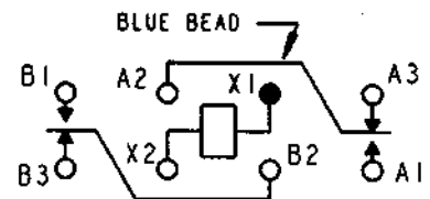
TERMINAL VIEW
