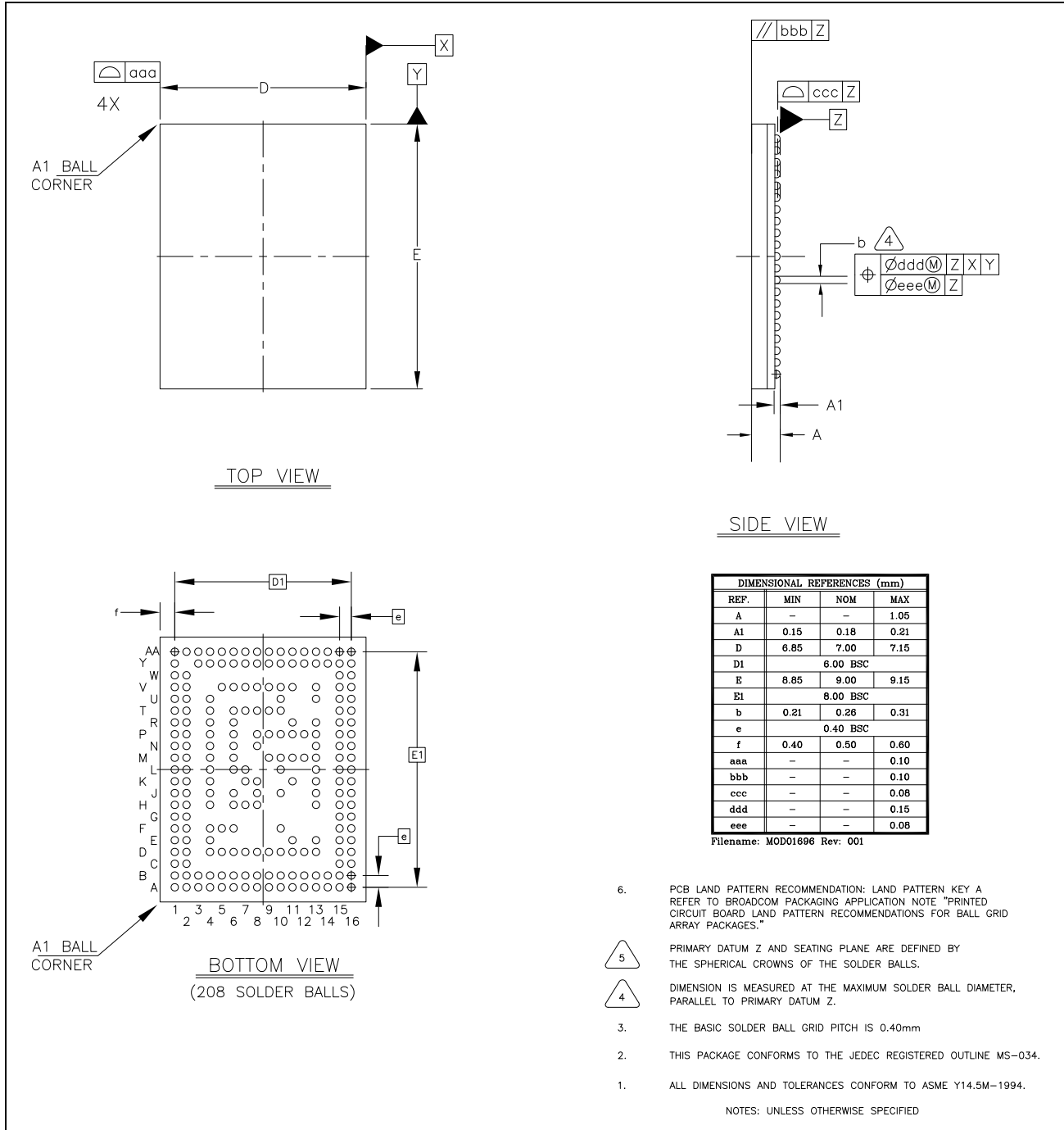
Figure 55: 208-Ball FCBGA Package Mechanical Information
