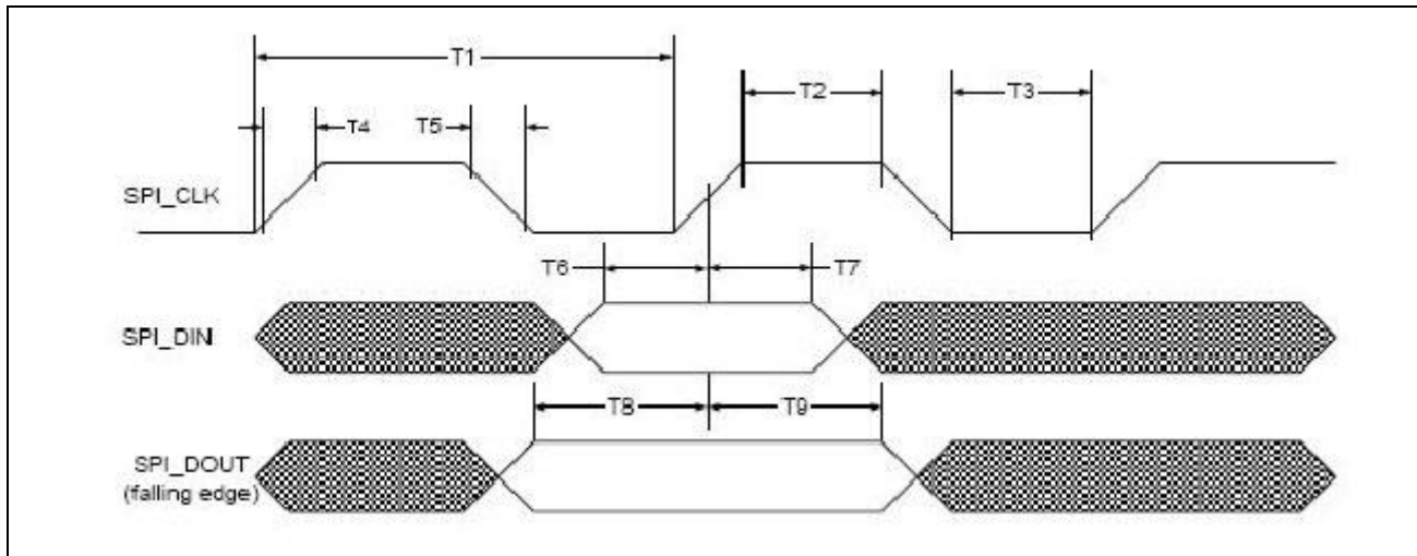
Figure 50: gSPI Timing
