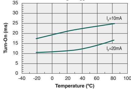
Typical Turn-On Time vs. Temperature ( I_L=1\text{A}_{DC} )
