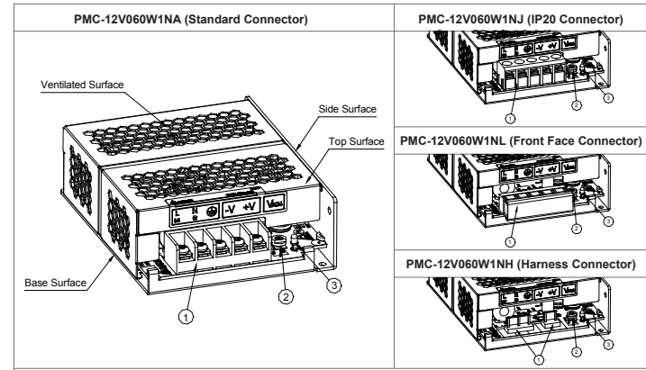
Fig. 1. Device Descriptions
