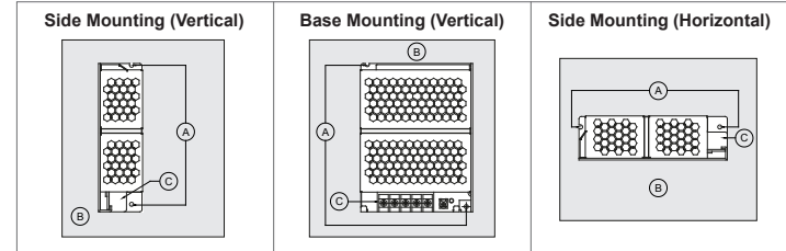
Fig. 2. Mounting Orientation
