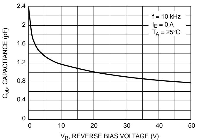
Figure 9. Output Capacitance
