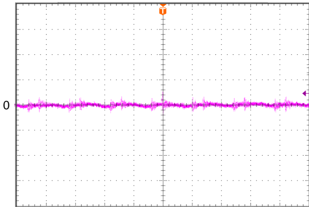
Figure 10: Input reflected ripple current, i_s , through a 12\ \mu\text{H} source inductor at nominal input voltage ( V_{\text{in}}=48\text{V} ) and rated load current ( 5\text{mA/div} , 2\text{us/div} )
