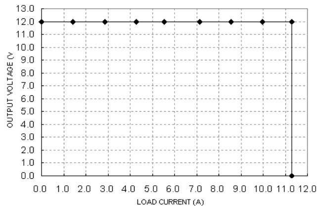
Figure 13: Output voltage vs. load current showing typical current limit curves and converter shutdown points ( V_{\text{in}}=48\text{V} )
