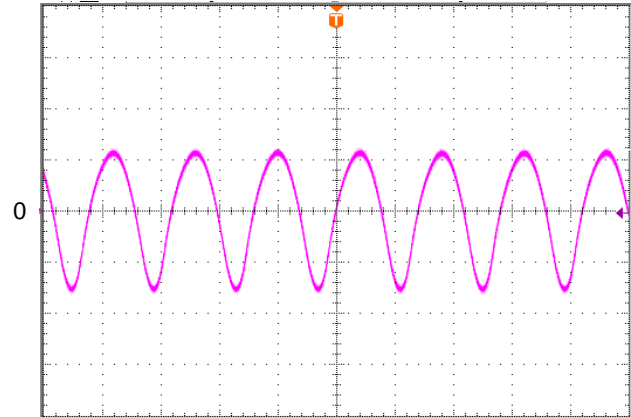
Figure 9: Input Terminal Ripple Current, i_c , at full rated output current and nominal input voltage ( V_{\text{in}}=48\text{V} ) with 12\ \mu\text{H} source impedance and 33\ \mu\text{F} electrolytic capacitor ( 250\text{mA/div} , 2\text{us/div} )
