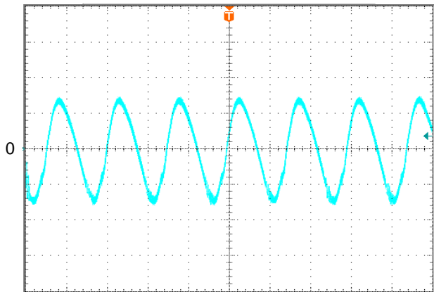
Figure 12: Output voltage ripple at nominal input voltage ( V_{\text{in}}=48\text{V} ) and rated load current ( I_o=9\text{A} ) ( 20\text{mV/div} , 2\text{us/div} ). Load capacitance: 1\ \mu\text{F} ceramic capacitor and 10\ \mu\text{F} tantalum capacitor. Bandwidth: 20 MHz. Scope measurements should be made using a BNC cable (length shorter than 20 inches). Position the load between 51 mm to 76 mm (2 inches to 3 inches) from the module
